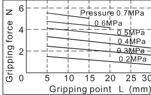
HFZ10\HFK10
