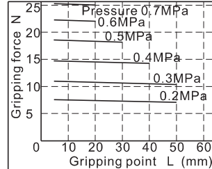
HFZ10\HFK10
