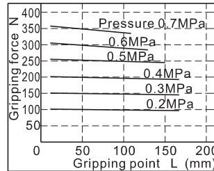
HFZ40\HFK40
