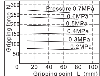
HFZ40\HFK40
