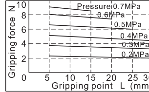
HFZ10\HFK10
