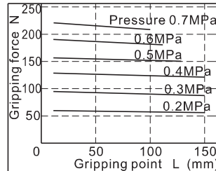
HFZ40\HFK40
