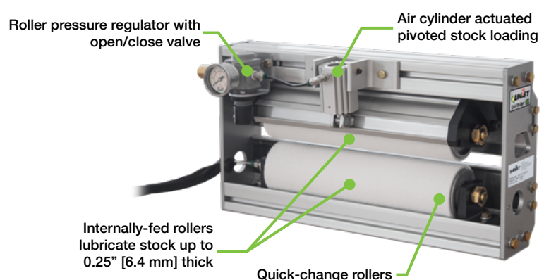
Single roller unit shown above. Lubricators with multiple roller sets have guards on both entry and exit sides.
